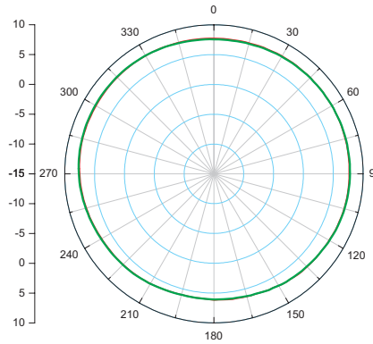
Azimuth Pattern
