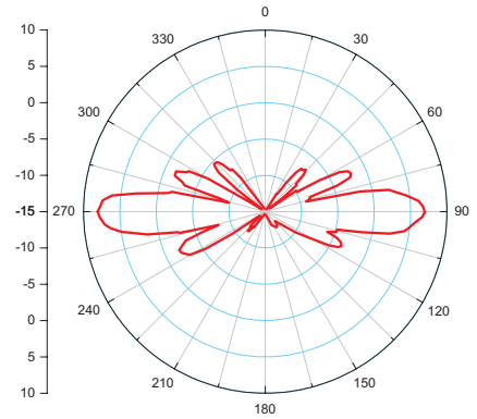
Elevation Pattern
